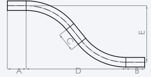
Offset Long Radius Bend
