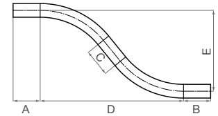
Offset Long Radius Bend
